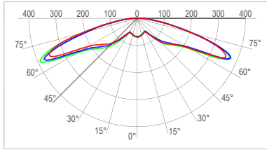
cd/klm — C0 - C180 — C90 - C270 — C50 - C230
